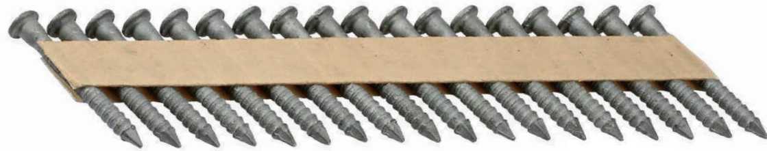
34° Positive placement nails / 35° Anchoring paper collated strip nails big head
