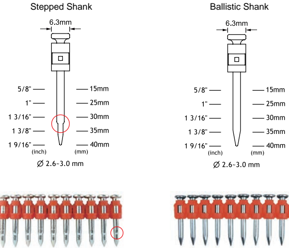
■ Heat-Treated Plastic Collated Concrete Nails For C3040
