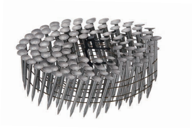
PC Drywall Coil Nail Shank Diameter \varnothing 2.5mm Length 38mm
