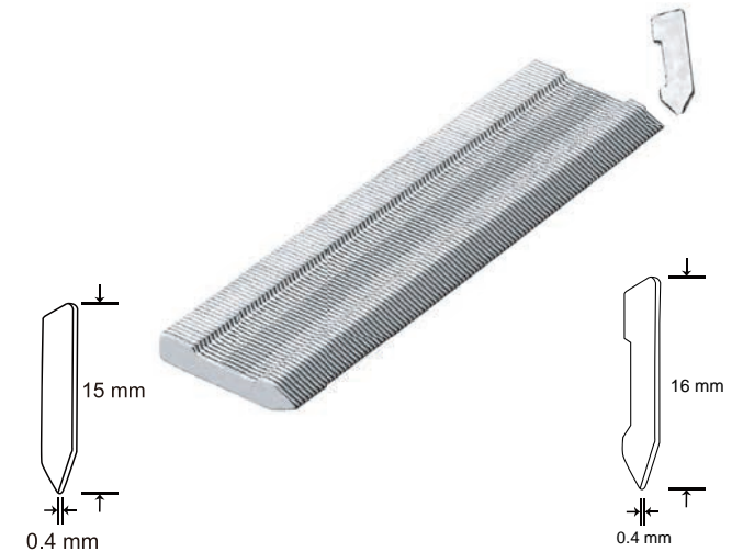
Arrow Head Tab - Fletscher type
